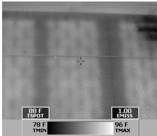
Vertical grout columns @ 40" O.C., top bond beam & double column at wall joint.
