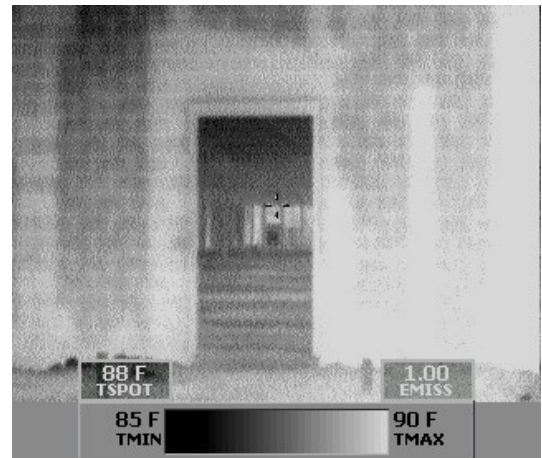
View of incomplete grouting around door jamb.
